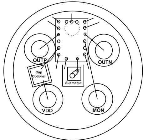
2) 5 pin TO bonding for PIN with fast IMON
