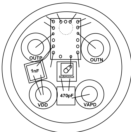
3) 5 pin TO bonding for APD w/o IMON
