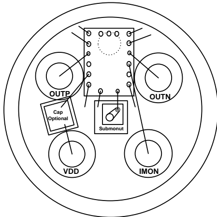
1) 5 pin TO bonding for PIN with precision IMON
