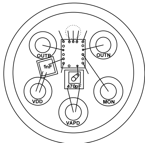
4) 6 pin TO bonding for APD with fast IMON
